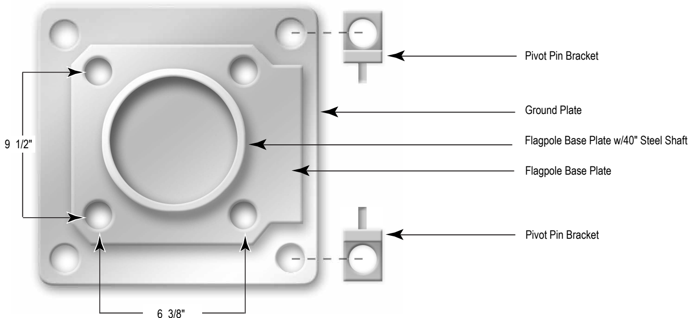
Top View
